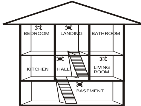
FIGURE 2 - 2/3 STOREY DWELLING
