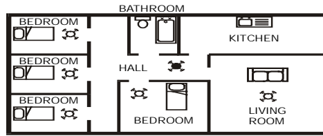
FIGURE 2 - 2/3 STOREY DWELLING
